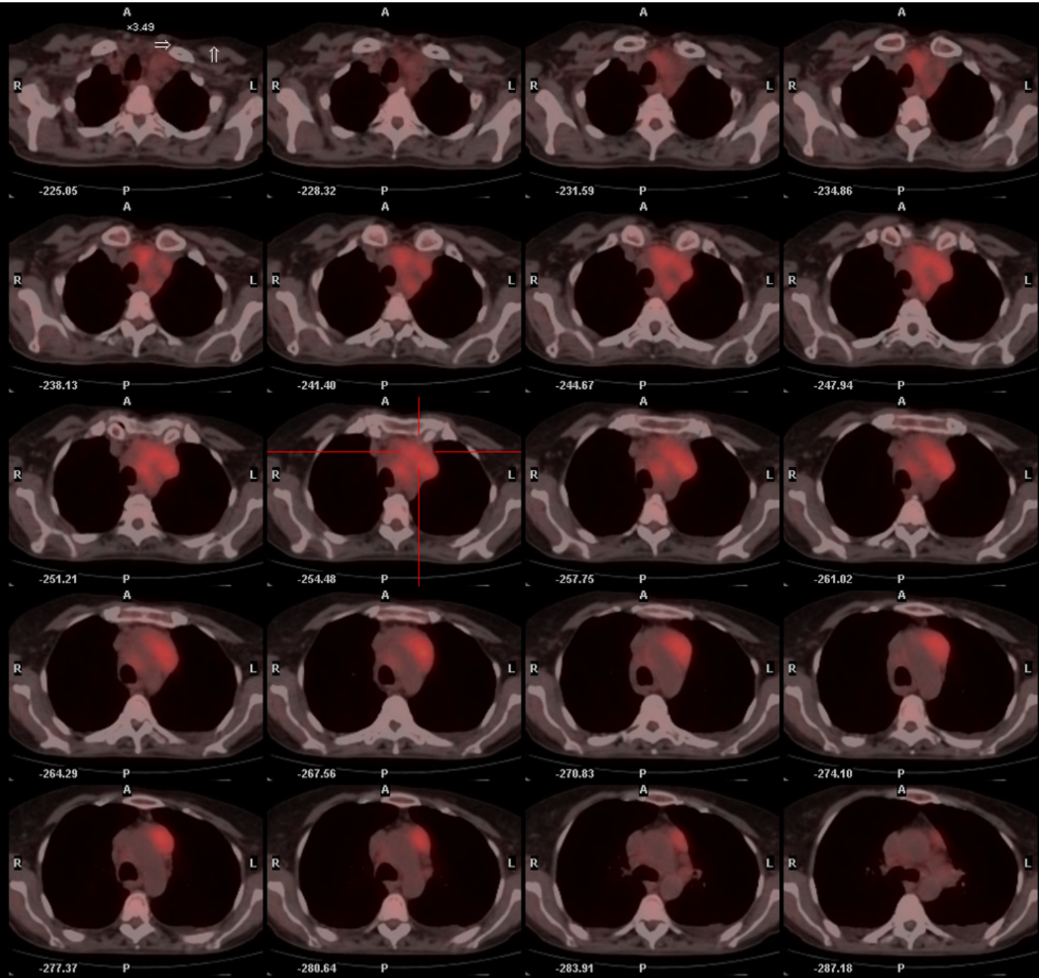
Fused Transaxials
